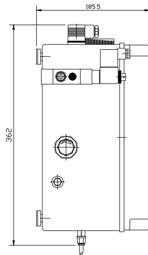
DIMENSIONS UCGF
