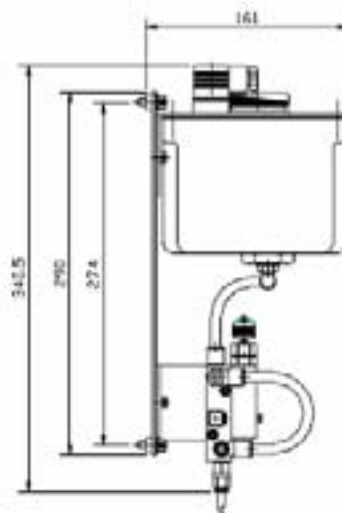
ENCOMBREMENTS AGSG-SE
