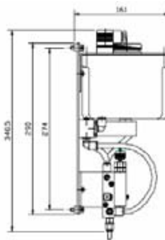
ENCOMBREMENTS AGGF-SE
