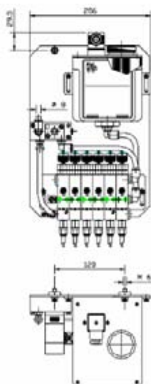
AFMETINGEN AGGF-SE
