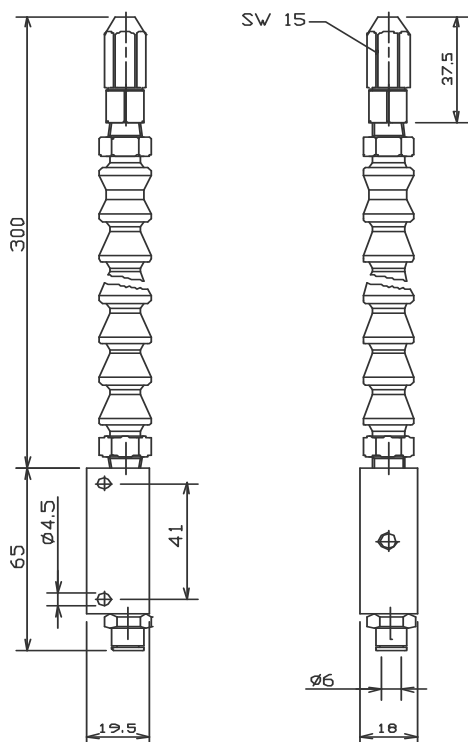
Code 70.100.0 FLEXIBEL LOCLINE ZONDER MAGNEET FLEXIBEL LOCLINE SANS AIMANT
